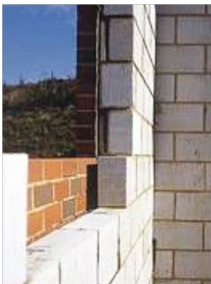
Modern cavity walls under construction.
